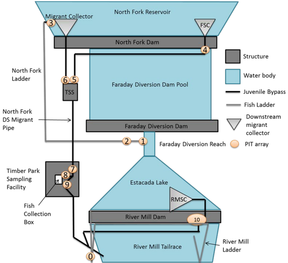
Figure 5. Schematic of PIT antenna array at the Clackamas Hydro Project. FSC = Floating surface collector; TSS = Tertiary screen structure; RMSC = River Mill surface collector (figure provided by Portland General Electric).
